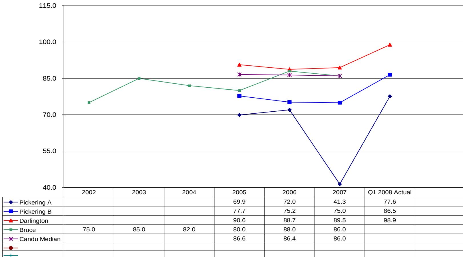
Capacity/Capability Factor (%)
